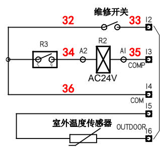
BeaconII Board 接线
